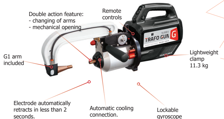
Supplied with: G1 arm, motorised overhanging arm with pulley (See next page)
